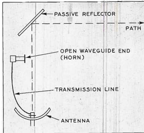
FIG. 7B. Horn located at passive reflector site.
