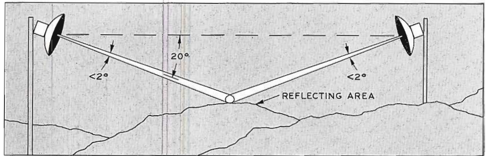
FIG. 3. Antennas approximately 20 degrees off path, yet reflection yields greater signal at receiver than was received in either Fig. 1 or Fig. 2. If either antenna "alone" is oriented along path, signal received will be weaker than reflection shown.
