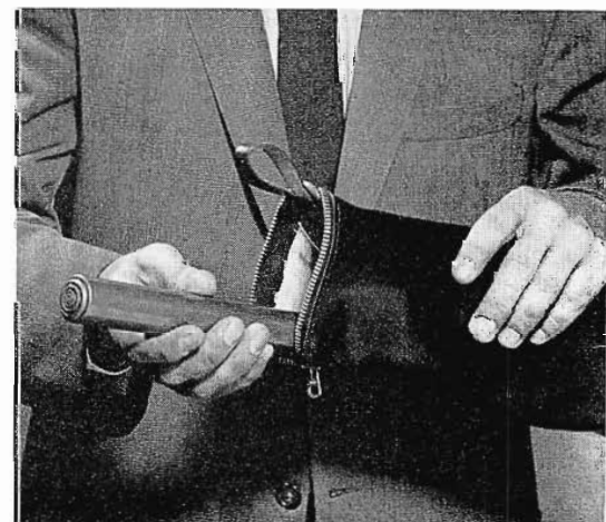
FIG. 3. The complete microphone-amplifier combination—together with earpiece, jack and 25-foot cable—is carried in a small zippered bag.
