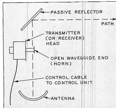
FIG. 7C. Horn located at passive reflector site.
