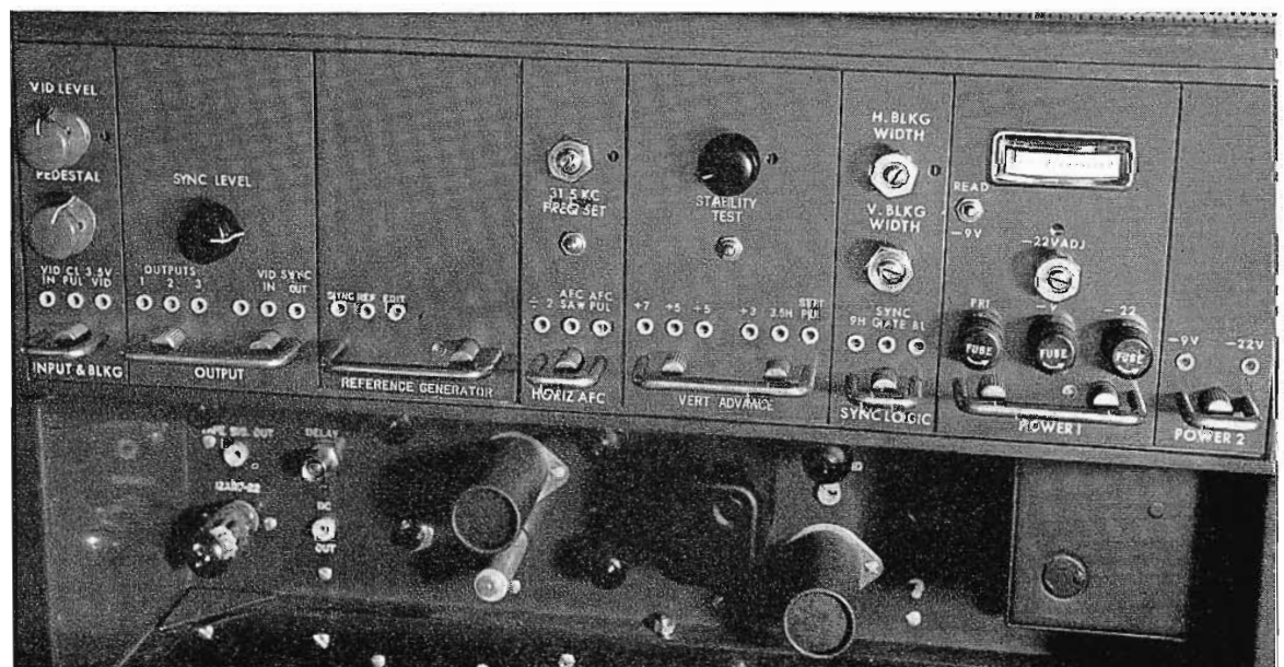
FIG. 5. The sync separation function is contained in this transistorized reference generator module, third unit from the left in the processing amplifier. This module also provides reference and edit pulses.
