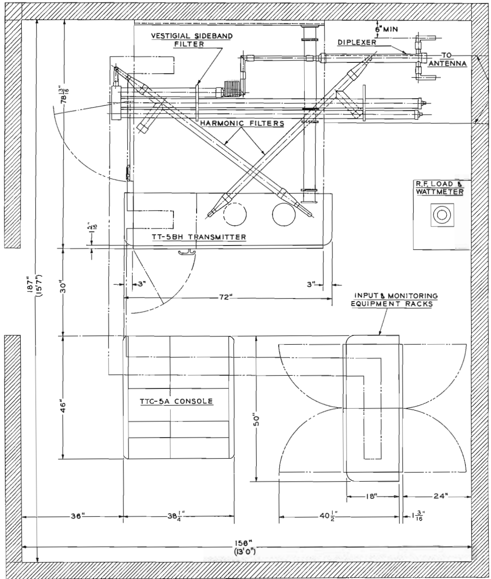
FIG. 6. Typical floor plan for TT-5BH.
