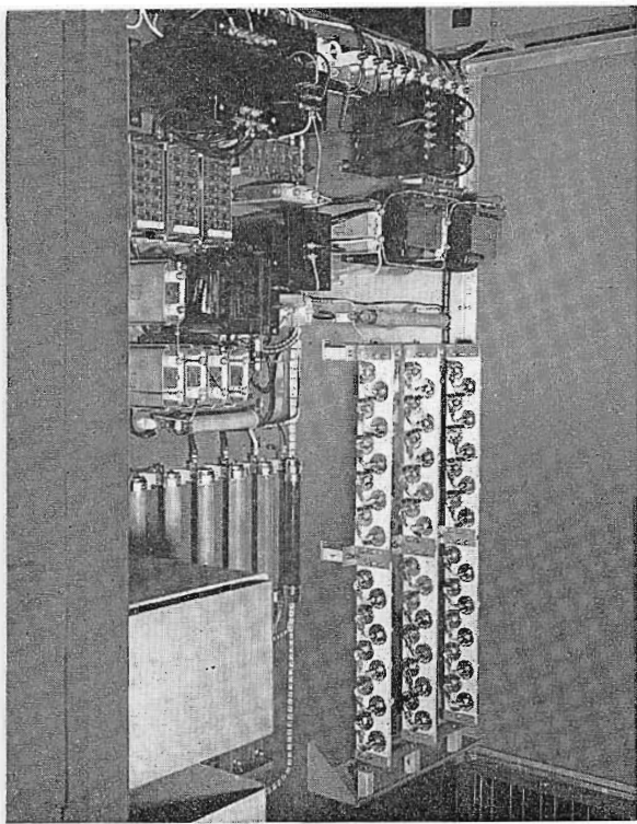
FIG. 4. Interior view of rectifier enclosure. High voltage silicon rectifiers are mounted on rear panel, easily accessible from aisle. They extend range of operating temperature and increase reliability of operation.
