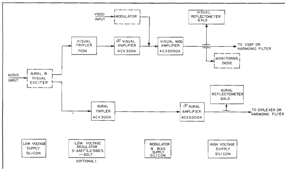
FIG. 5. Block diagram of TT-5BH.
