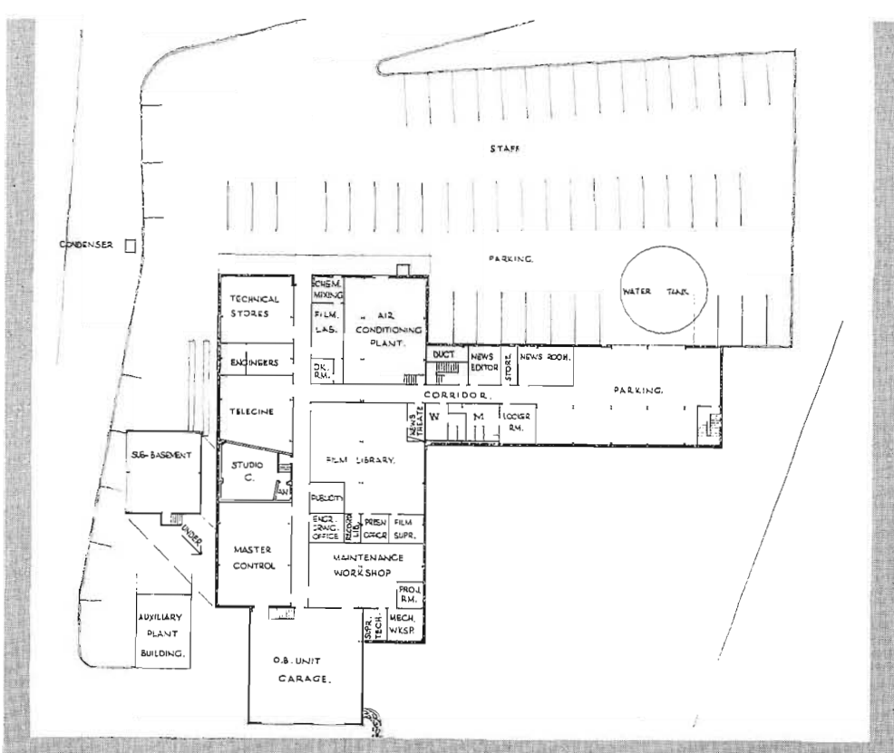
FIG. 4. The layout of the Central Technical Area can be seen clearly in the architect's simplified basement floor plan.
