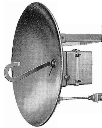
FIG. 1. Antennas less than 6 degrees off path, yet virtually no signal is obtained at receiver.
