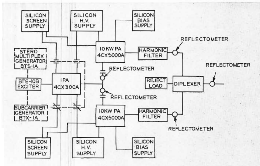
FIG. 9. Block diagram of BTF-20D Transmitter.
