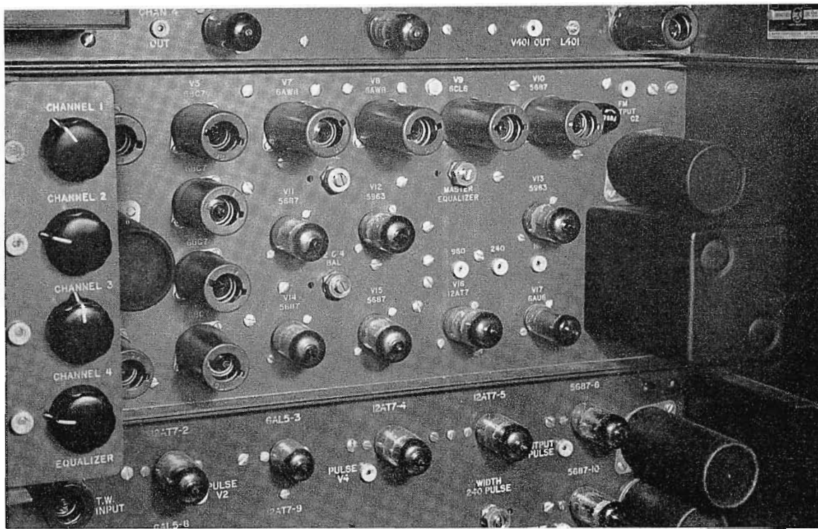
FIG. 4. This chassis incorporates the functions of both the 4 by 2 and 2 by 1 switchers found in the TR-11's senior partner, the TRT-1B TV Tape Recorder. In the re-design of this unit the sync separation function has been relegated to another chassis.
