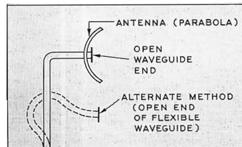
FIG. 7A. Horn located at parabolic antenna site.
