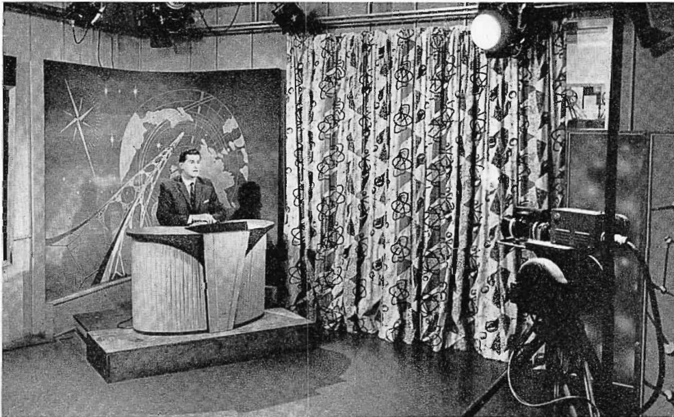
FIG. 11. Studio C is 21 feet by 21 feet and is used for the presentation of News and Weather Bulletins together with simple live commercials and interview-type programmes. This Studio is equipped with a TK-21 vidicon camera used in conjunction with a zoom lens. The camera and lens have complete remote control of pan, tilt, focus, iris and zoom. Preset lighting and the special camera facilities allow for unattended operation in this Studio.
