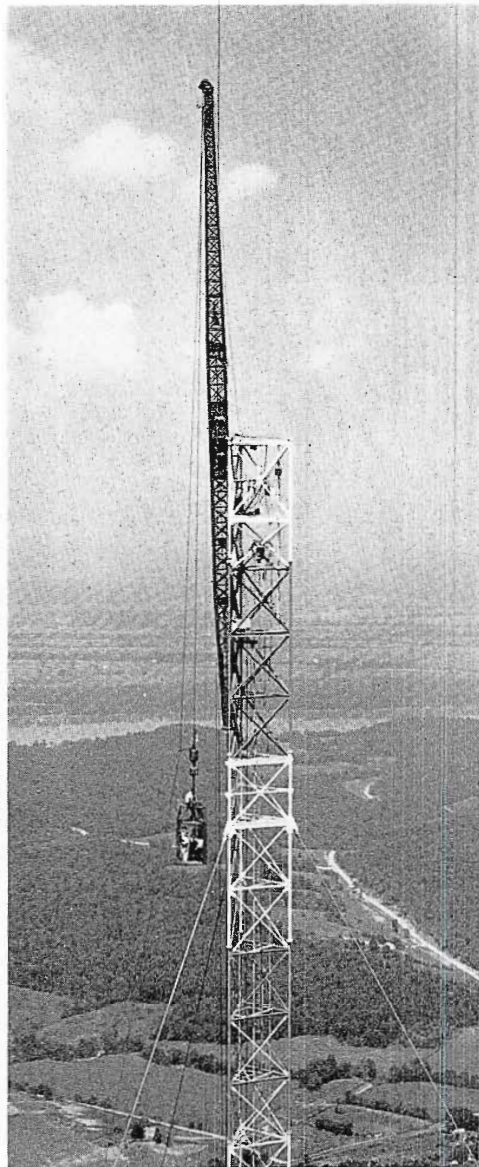
FIG. 4. At the site, 30-ft. sections were assembled and painted on the ground then hoisted aloft and bolted into place. Special hoisting equipment used consisted of a heavy boom (gin pole) that "walked" up the tower as it grew.
