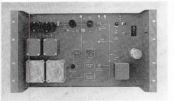
FIG. 7. Stereo Subcarrier Generator, Type BTS-1A—an optional accessory for FM stereo operation.
