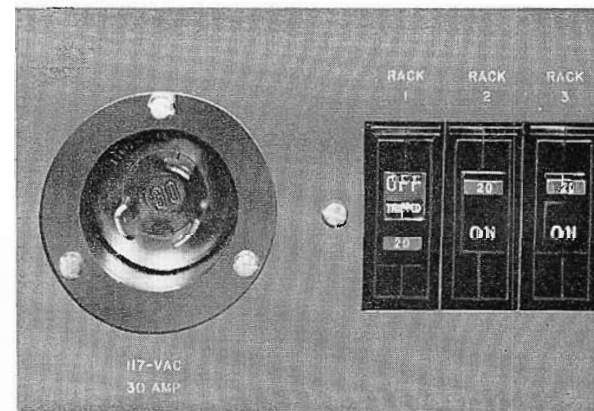
FIG. 8. Low power consumption in the TR-11 permits a single a-c power feed to be supplied to one main connector. Three a-c breakers evenly distribute power throughout the recorder.
