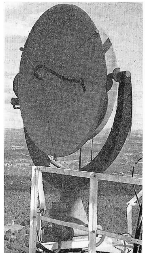
FIG. 18. A TF-55A rotatable mount with a 6-foot reflector can be seen on the 200-foot level on the tower. The unit is remotely controlled from the master control room.
