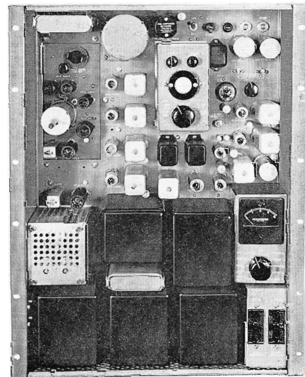
FIG. 6. Type BTE-10B Exciter including self-contained semiconductor d-c power supply is housed on hinged vertical chassis which provides instant accessibility to all components and circuits. The built-in scope permits constant observation of the AFC circuits. The meter is used to check all important circuit constants.
