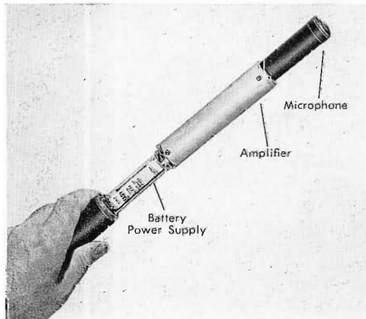
FIG. 2. View of BN-10A with protective barrel removed to show construction and elements.
