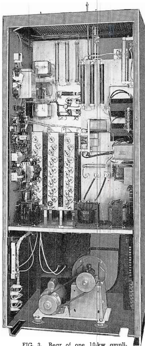
FIG. 3. Rear of one 10-kw amplifier. Note blower at bottom. Each PA has its own plate transformer and grid bias supply.
