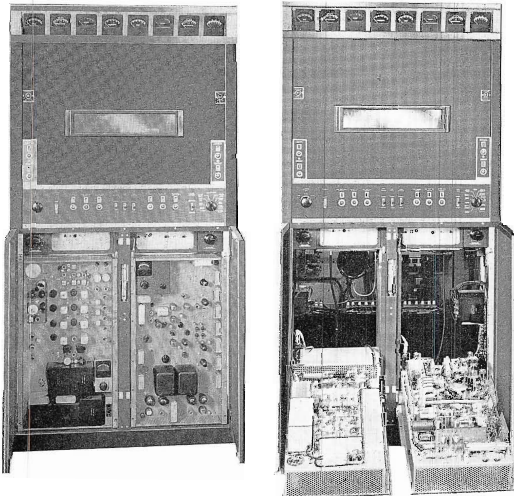
FIG. 3. Note accessibility from front of newest RCA TV Transmitter. At left, "Dutch" doors open to reveal exciter and modulator chassis. At right, these chassis, which are hinged on the bottom, are in lowered position to facilitate servicing. All important meters are mounted on a sloping panel at the top, with built-in lighting. Tuning and operating controls are mounted on waist-height panel above dutch doors.
